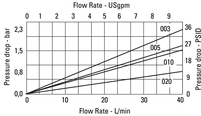
ORFM C-Pak Length 3
