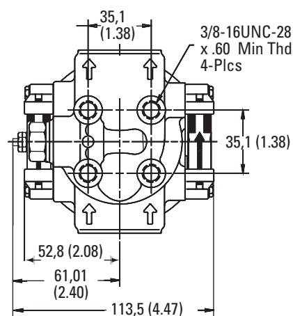
OFRP35 with optional electrical indicator
