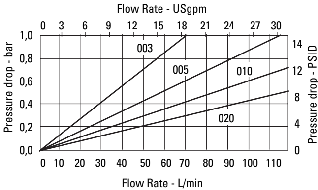
ORFM C-Pak Length 5
