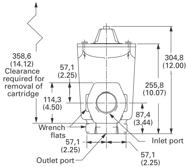
Threaded Ports
