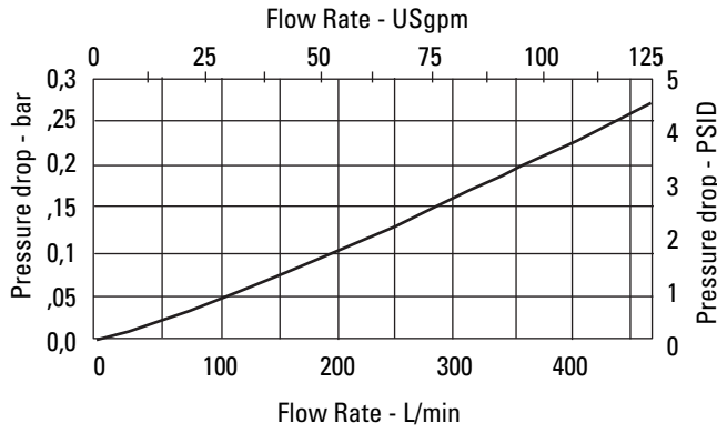
ORFM Length 5 Housing
