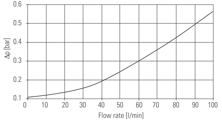
DHP 063/100
