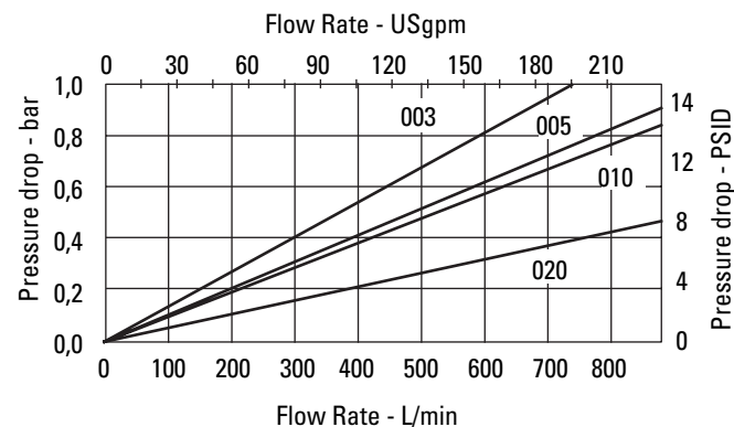
ORFM C-Pak Length 7
