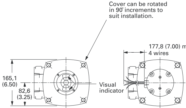
Mechanical Indicator
