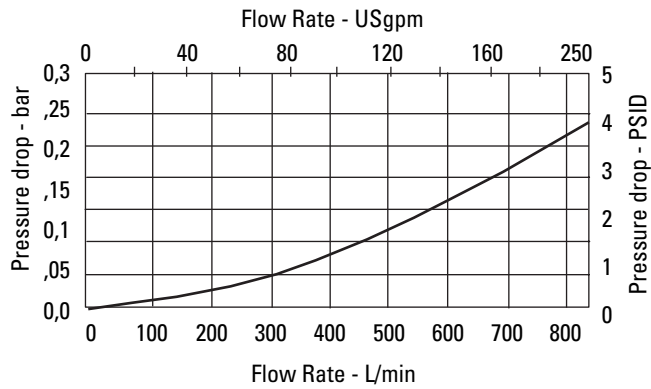
ORFM Length 6 & 7 Housing
