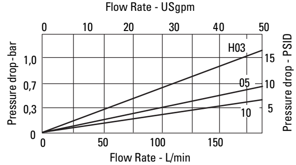
HF4P H-Pak Element Length 6
