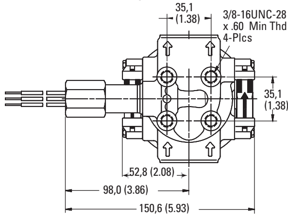
OFRP35 with optional electrical indicator
