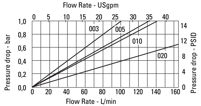
ORFM C-Pak Length 4
