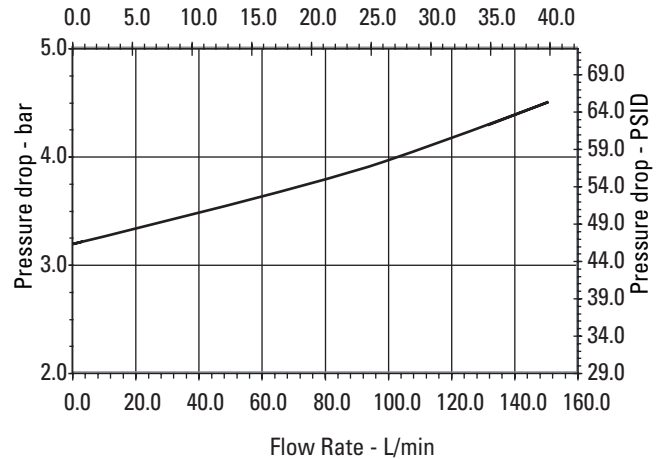
ORFM Length3 Bypass
