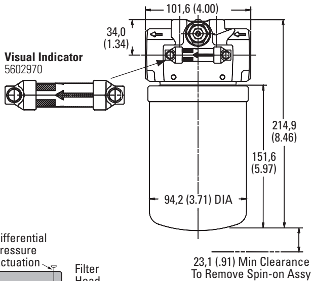
OFRP35 with B1 Length Filter Element
