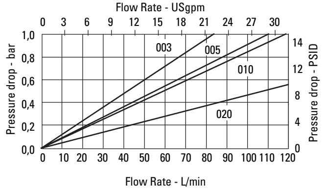
ORFM C-Pak Length 4
