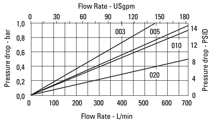
ORFM C-Pak Length 6
